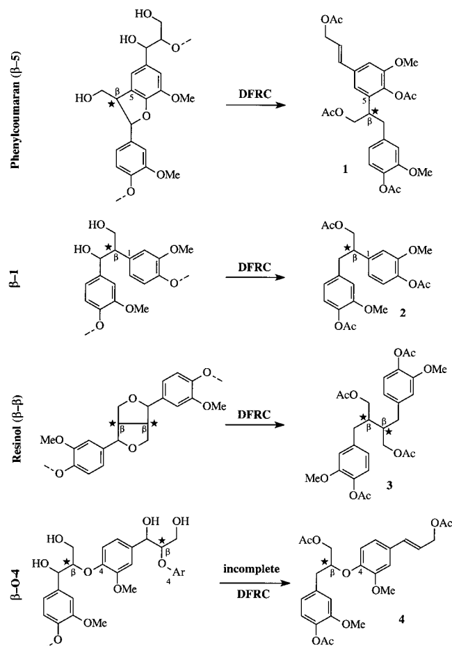
Figure 1. Dimeric DFRC products from various structural units in softwood lignins. Optical centers at \beta -carbons formed by radical coupling reactions during lignification are denoted with a \star . The \beta -O-4-dimer 4 is produced only in small amounts from incomplete ether cleavage.
